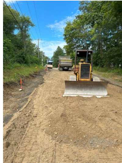
DPW staff working on drainage and road base upgrades.
